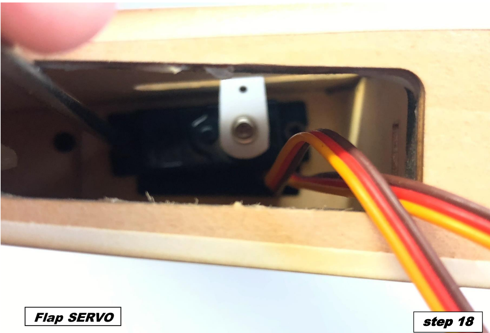
Flap SERVO
